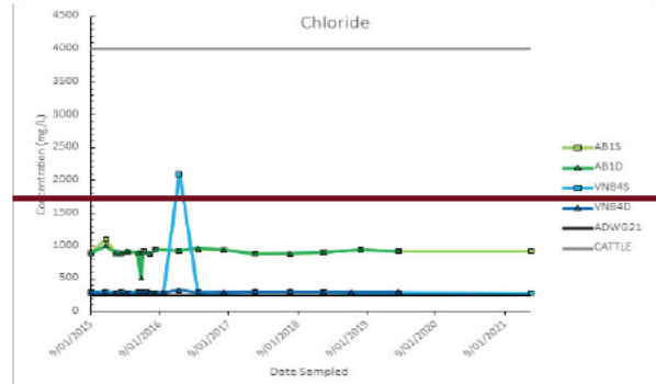
Figure 4-4: Chloride [Liveringa]
