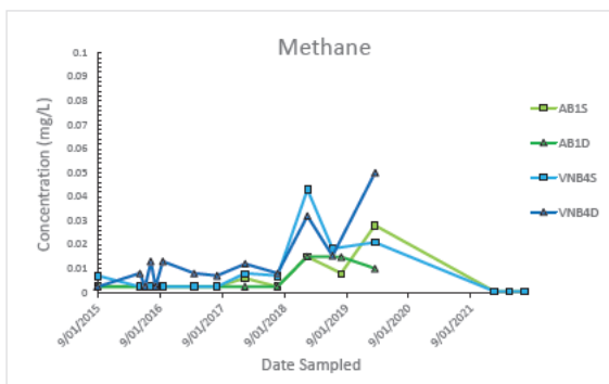
Figure 4-13: Methane [Liveringa]
