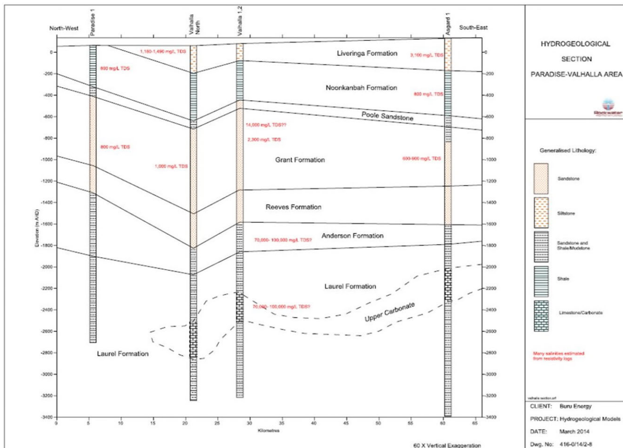
Figure 4-2: Hydrogeological Cross-Section
