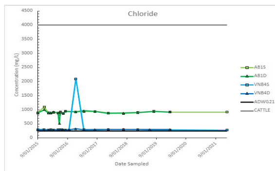
Figure 4-4: Chloride [Liveringa]
