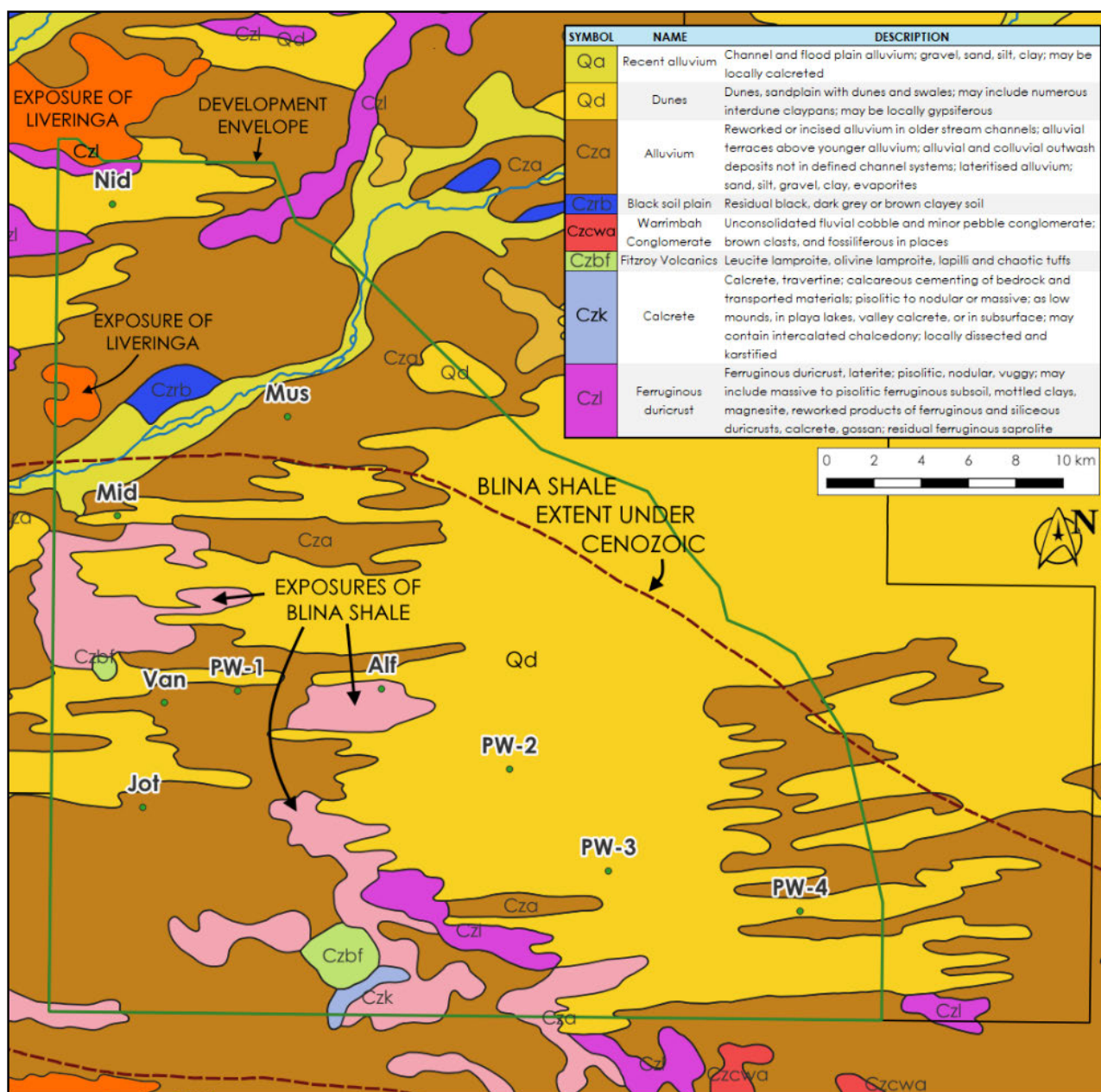
Figure 4-22: Supplemental Geology Map (Stewart et al., 2020)
