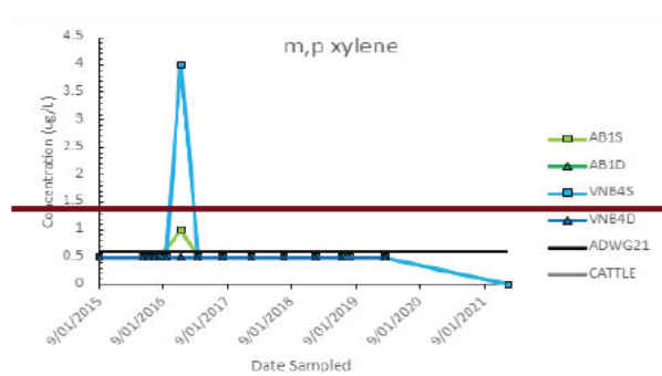
Figure 4-12: Xylene [Liveringa]
