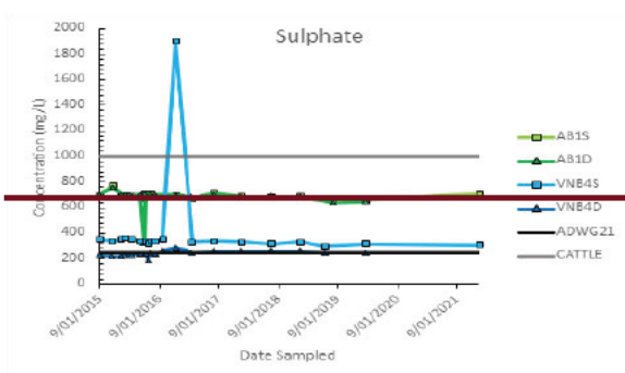
Figure 4-5: Sulphate [Liveringa]
