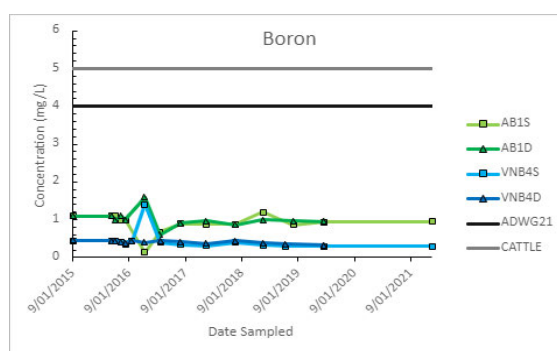
Figure 4-6: Boron [Liveringa]
