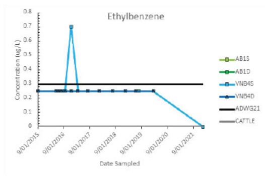
Figure 4-11: Ethylbenzene [Liveringa]
