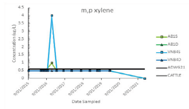
Figure 4-12: Xylene [Liveringa]
