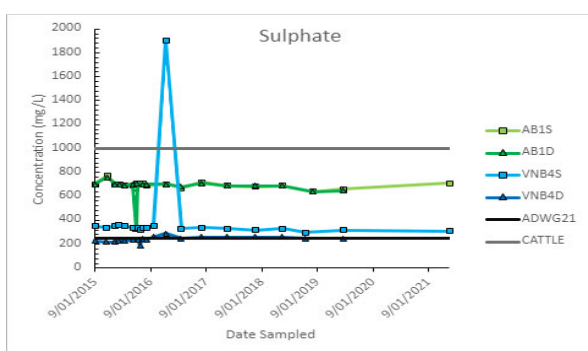
Figure 4-5: Sulfate [Liveringa]
