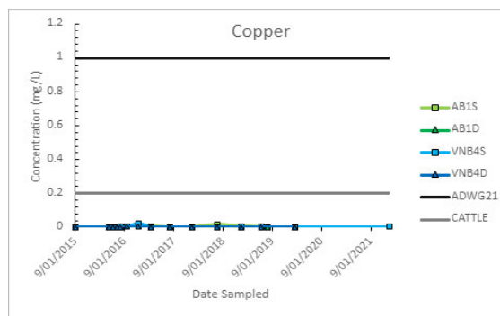
Figure 4-8: Copper [Liveringa]
