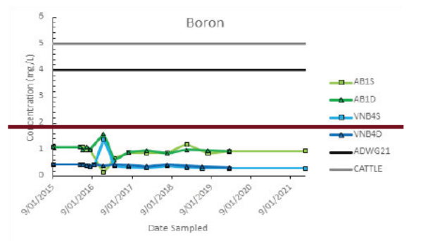
Figure 4-6: Boron [Liveringa]
