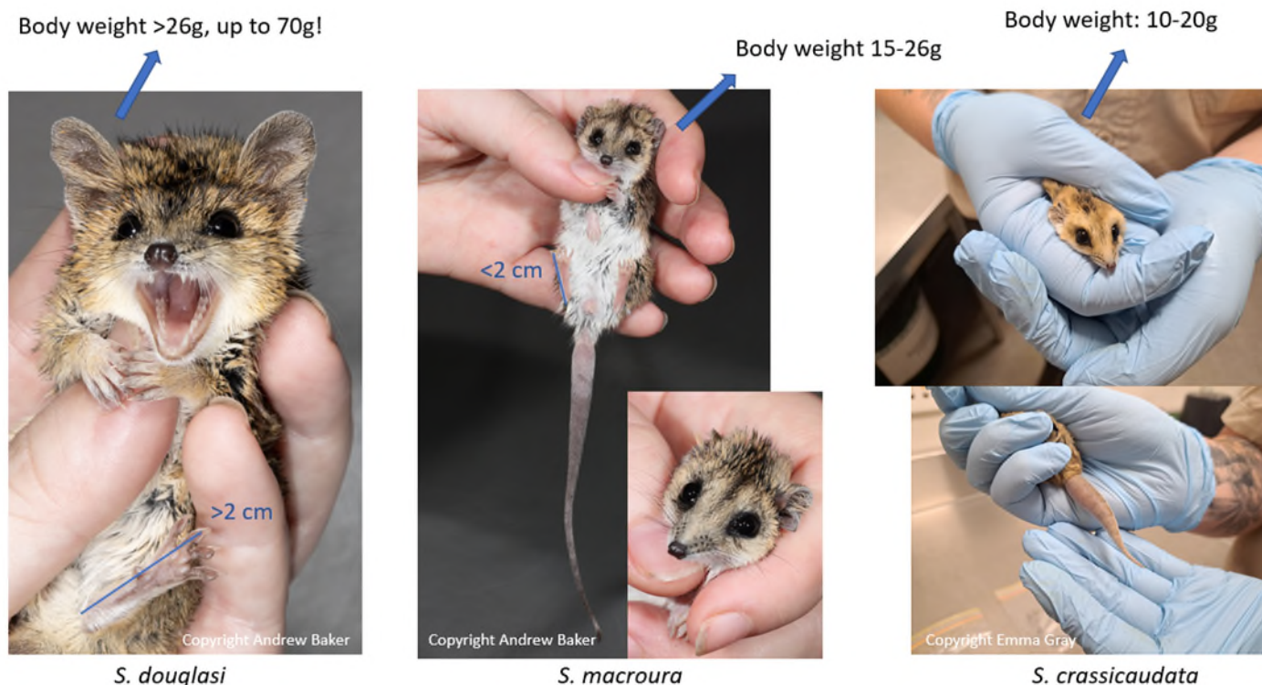
Diagram showing key differences between adult Smynthopsis species occurring in north-west Queensland.
